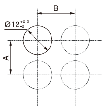
□ K12安装尺寸 / K12 Installation size
